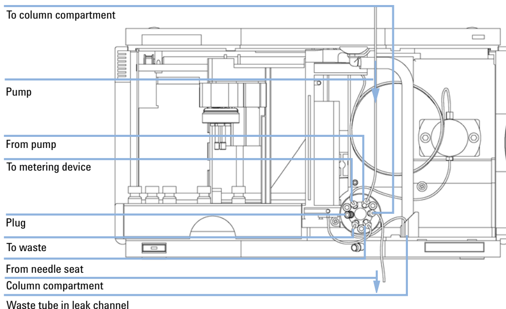
Figure 10 Hydraulic Connections
