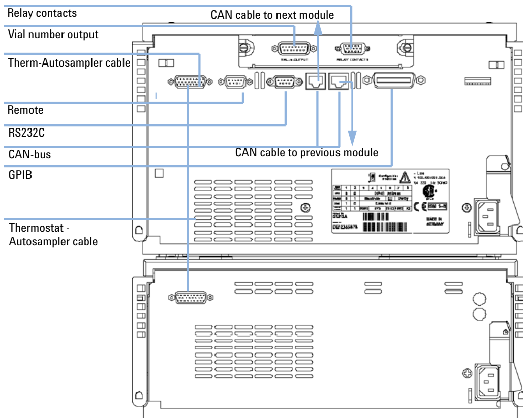
Figure 17 Electrical Connections
