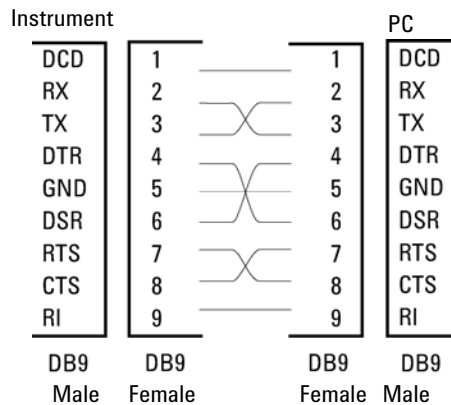
Figure 37 RS-232 Cable
