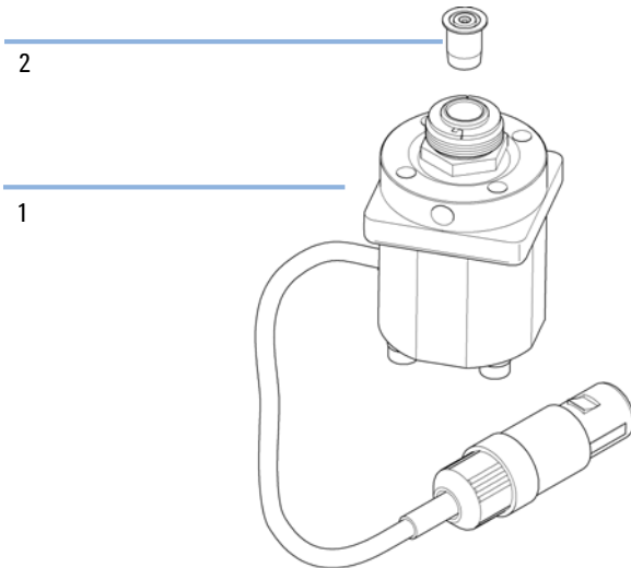
Figure 31 Active Inlet Valve Assembly
