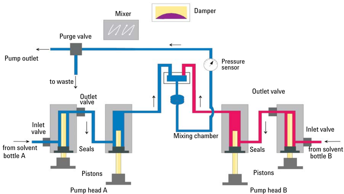
Figure 3 The Hydraulic Path of the Binary Pump with Bypassed Damper and Mixer
