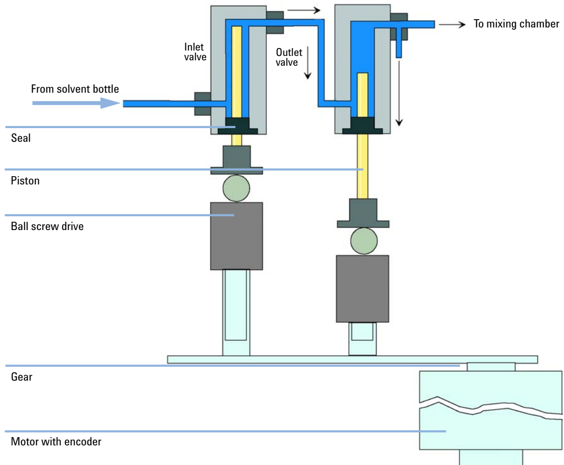
Figure 4 Pump head
